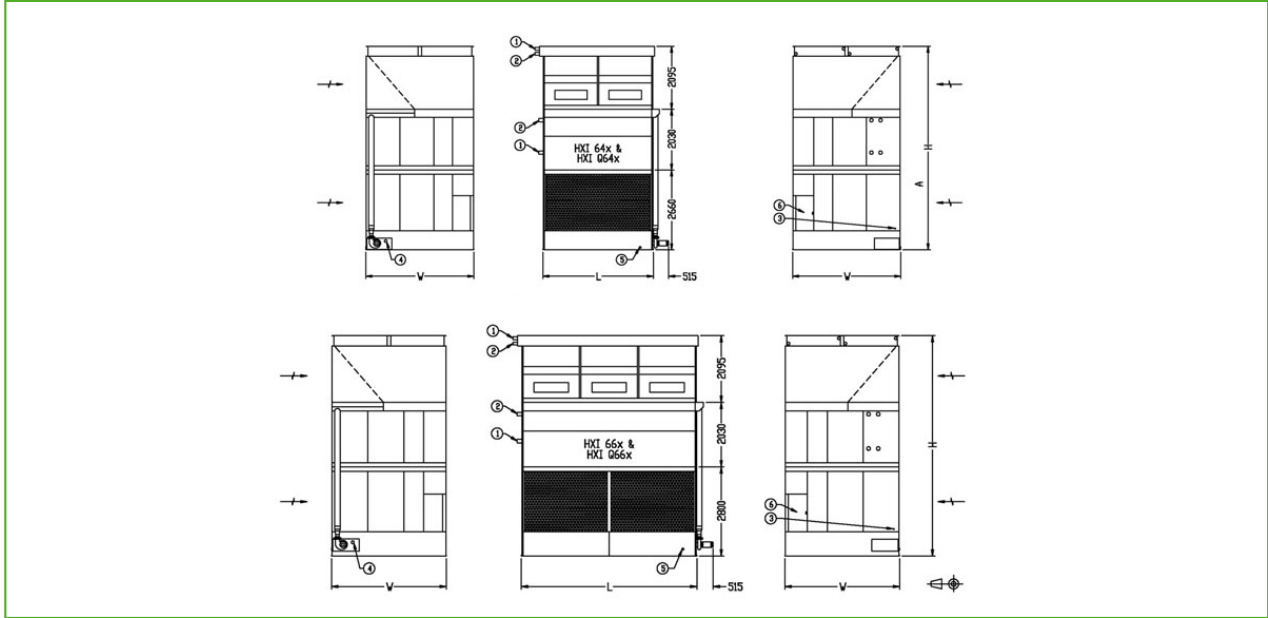
1. Inlet connection; 2. Outlet connection; 3. Make up ND25; 4. Overflow ND80; 5. Drain ND50; 6. Access door.
