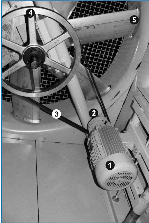
Drive system
